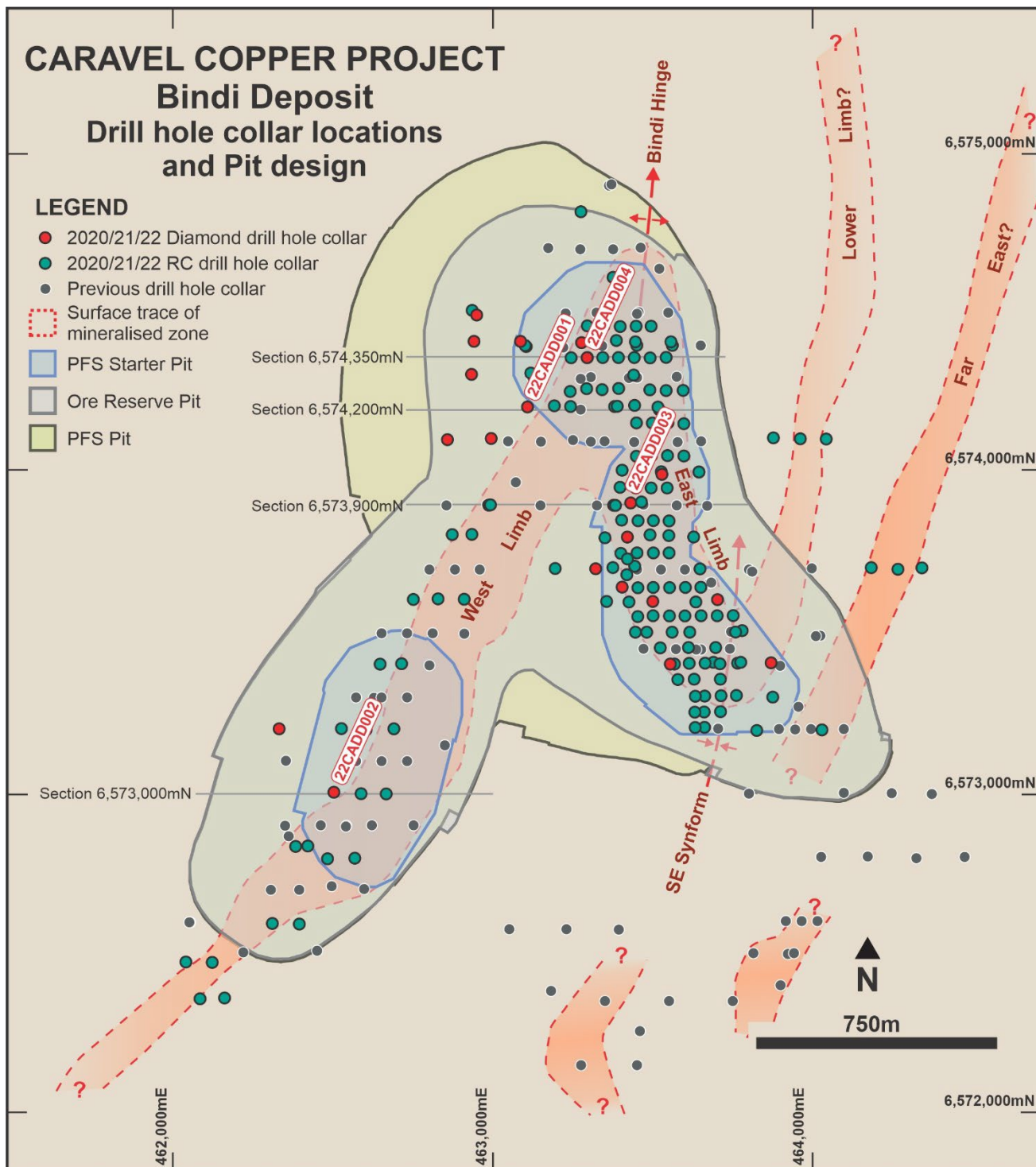
Figure 1: Drilling status plan of the Bindi copper deposit showing the locations of the reported diamond core drill holes. Drill holes from the 2021/22 program, previous drill collars, simplified geology and the 2022 PFS optimised pits are shown for reference.
