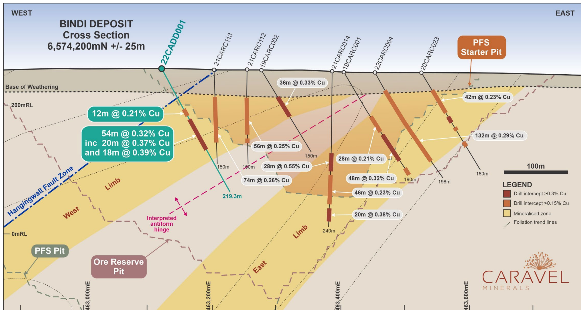
Figure 4: Schematic geological cross section of the Bindi Deposit West Limb (6,574,200mN) showing location of recent Diamond Core (CADD prefix) drill holes and mineralised intersections.
