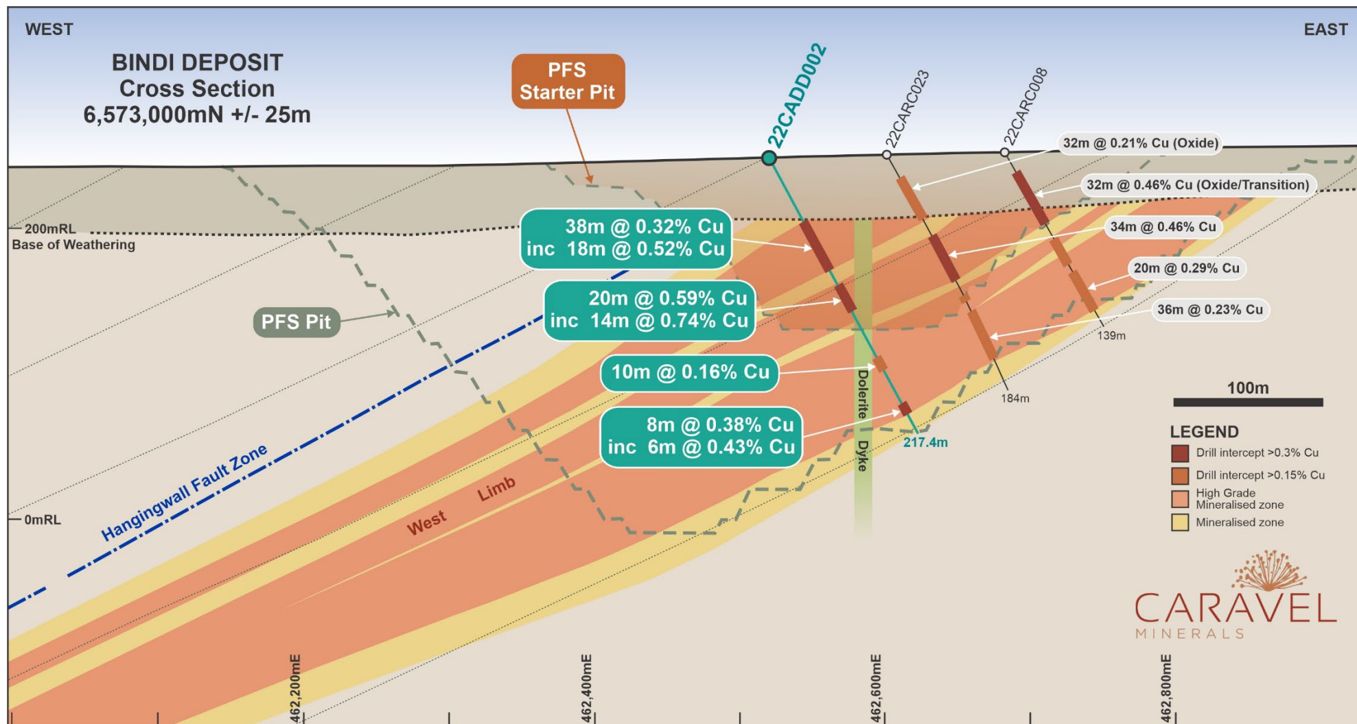
Figure 2: Schematic geological cross section of the Bindi Deposit West Limb (6,573,000mN) showing location of recent Diamond Core (CADD prefix) drill hole and mineralised intersections.
