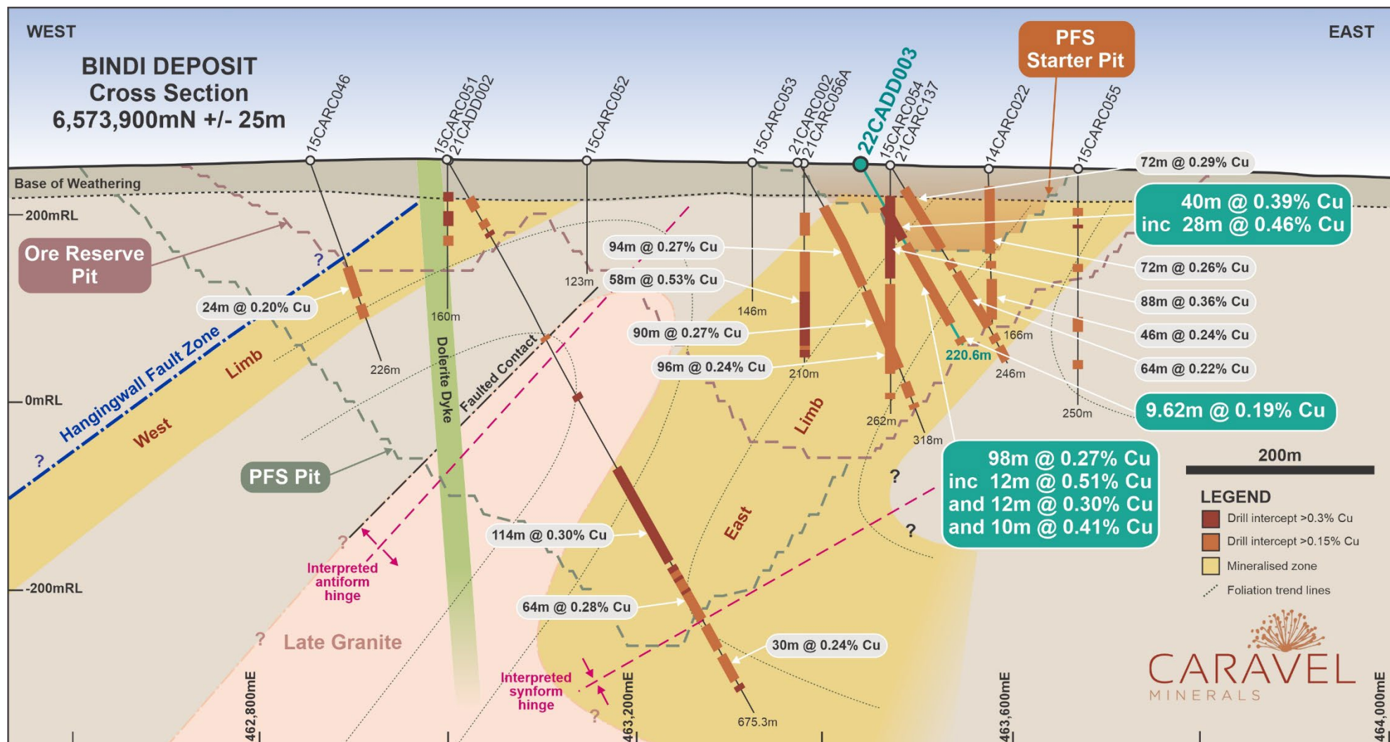
Figure 3: Schematic geological cross section of the Bindi Deposit East Limb (6,573,900mN) showing location of recent Diamond Core (CADD prefix) drill holes and mineralised intersections.
