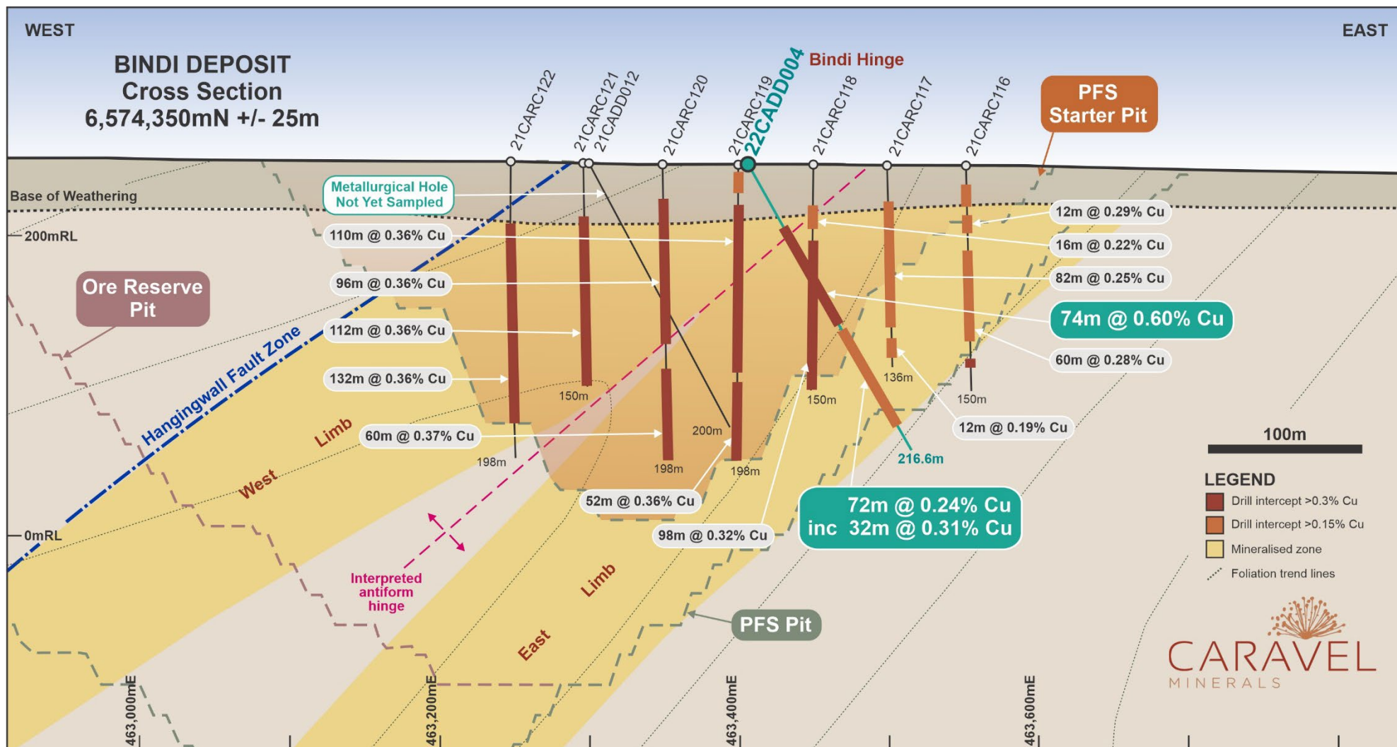
Figure 5: Schematic geological cross section of the Bindi Deposit Hinge Zone (6,574,350mN) showing location of recent Diamond Core (CADD prefix) drill holes and mineralised intersections.
