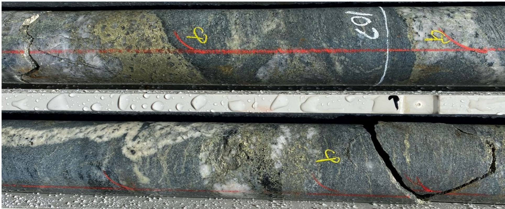
Figure 6: Diamond core from 22CADD004 (Bindi Hinge) 107-109m showing strong chalcopyrite stringer mineralisation.
