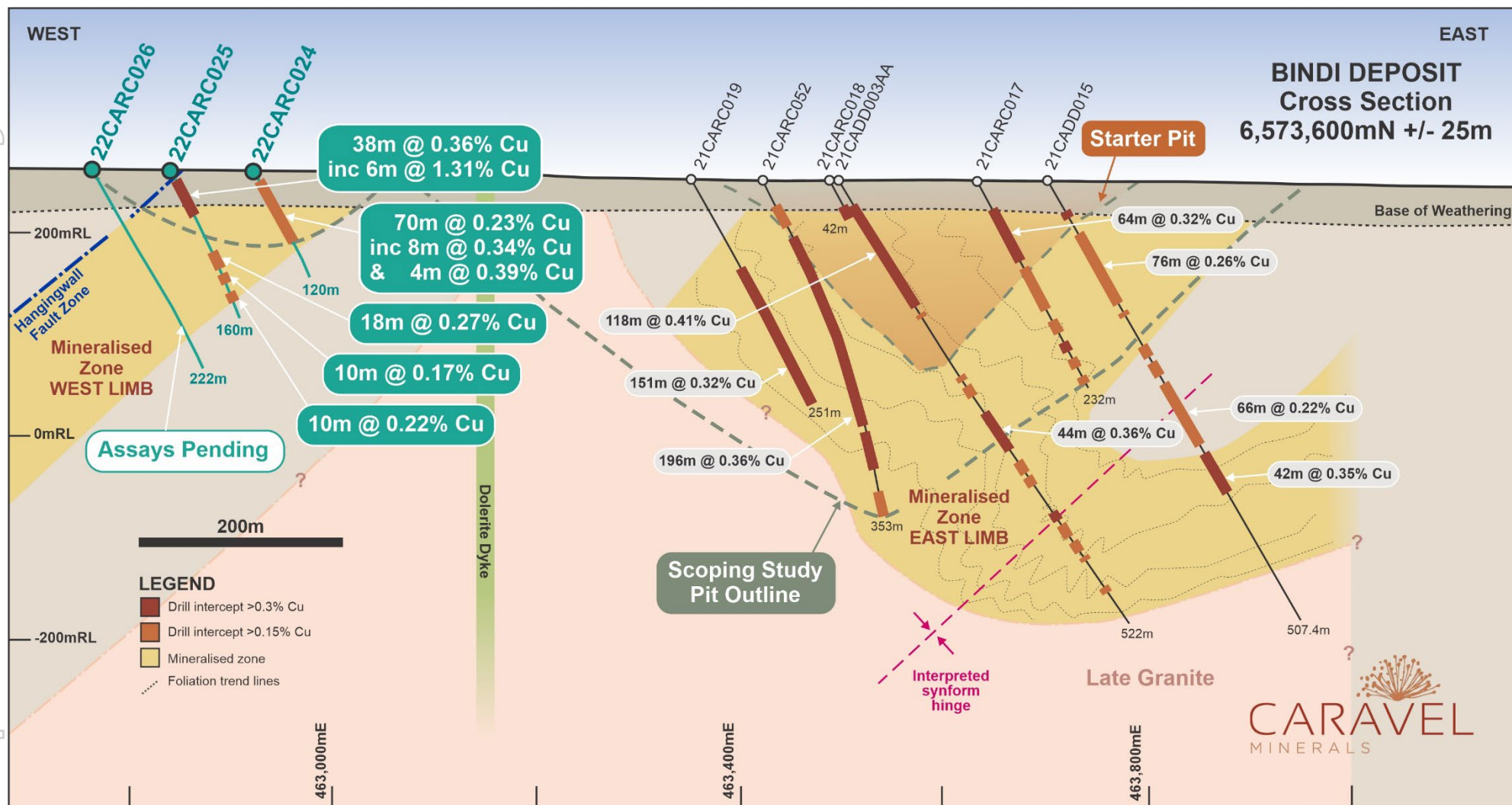
Figure 3: Schematic geological cross section of the Bindi Deposit (6,573,600mN) showing location of recent RC percussion (CARC prefix) drill holes and mineralised intersections.
