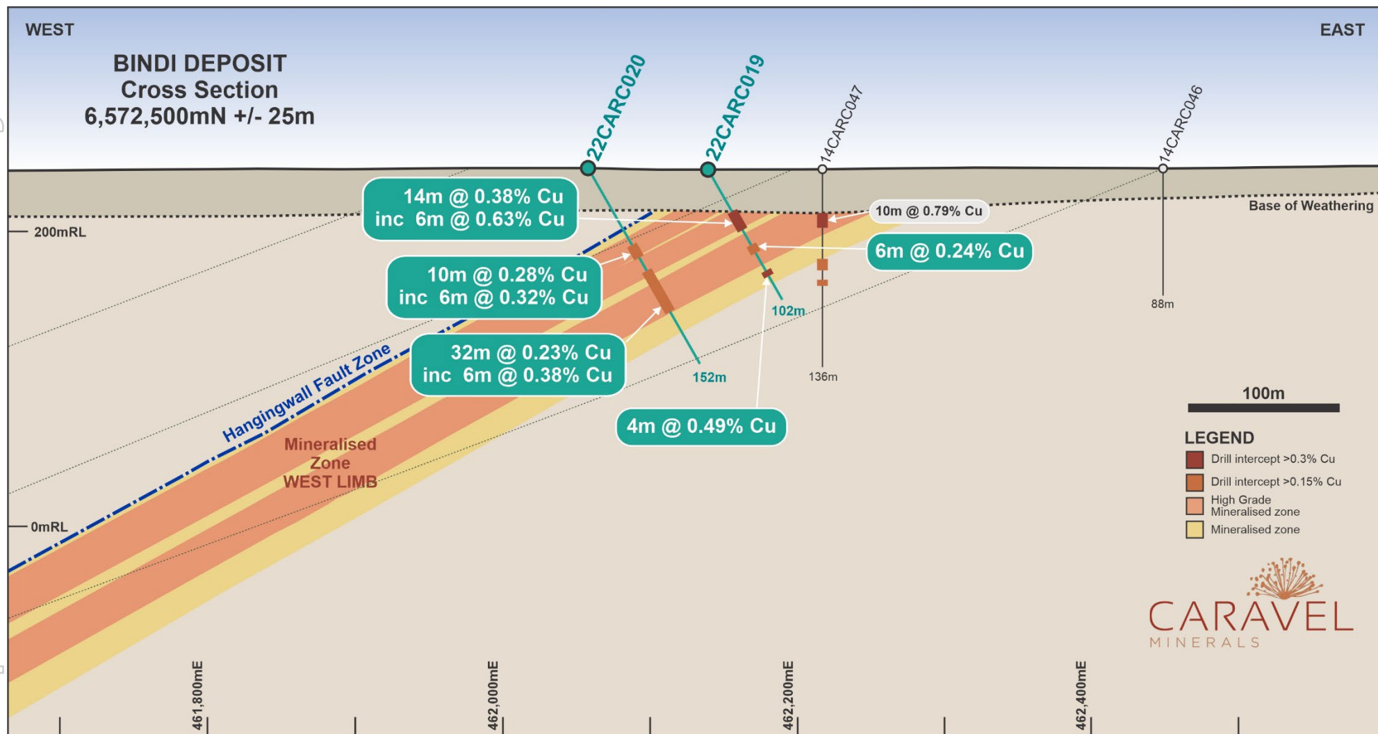
Figure 7: Schematic geological cross section of the Bindi Deposit (6,572,500mN) showing location of recent RC percussion (CARC prefix) drill holes and mineralised intersections.
