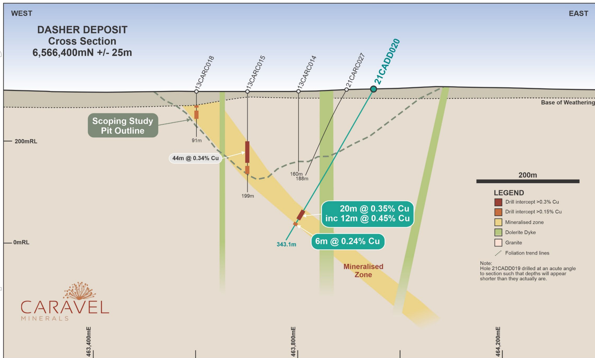
Figure 8: Schematic geological cross section of the Dasher Deposit (6,566,400mN) showing location of recent diamond core drill hole (CADD prefix) and previous RC percussion (CARC prefix) drill holes and mineralised intersections.
