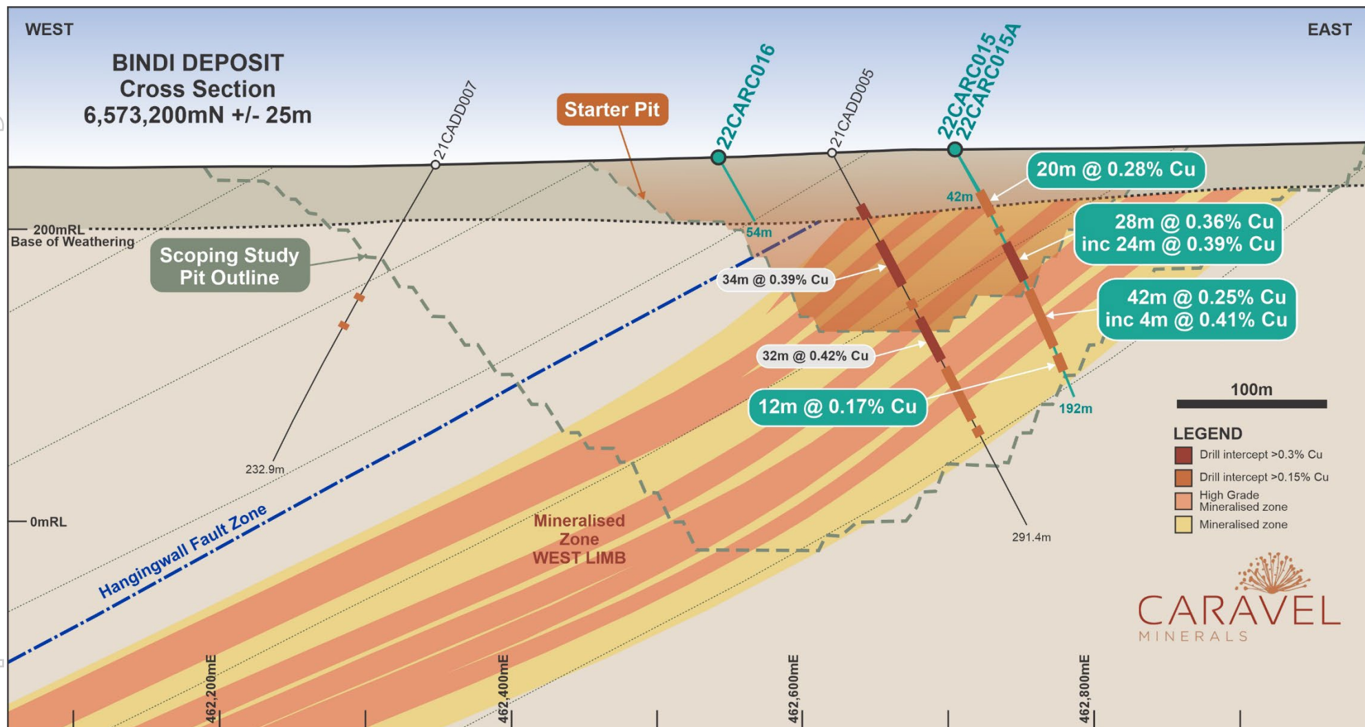
Figure 4: Schematic geological cross section of the Bindi Deposit (6,573,200mN) showing location of recent RC percussion (CARC prefix) drill holes and mineralised intersections.
