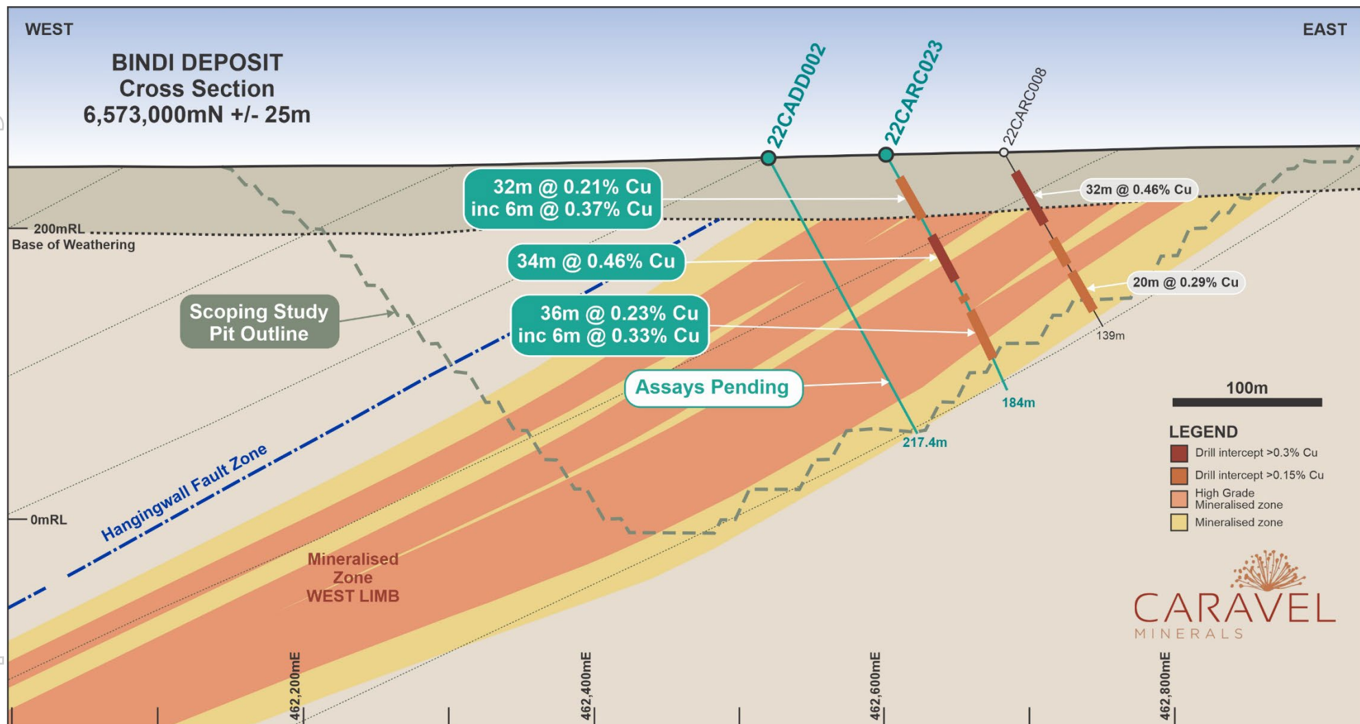
Figure 5: Schematic geological cross section of the Bindi Deposit (6,573,000mN) showing location of recent RC percussion (CARC prefix) drill holes and mineralised intersections.
