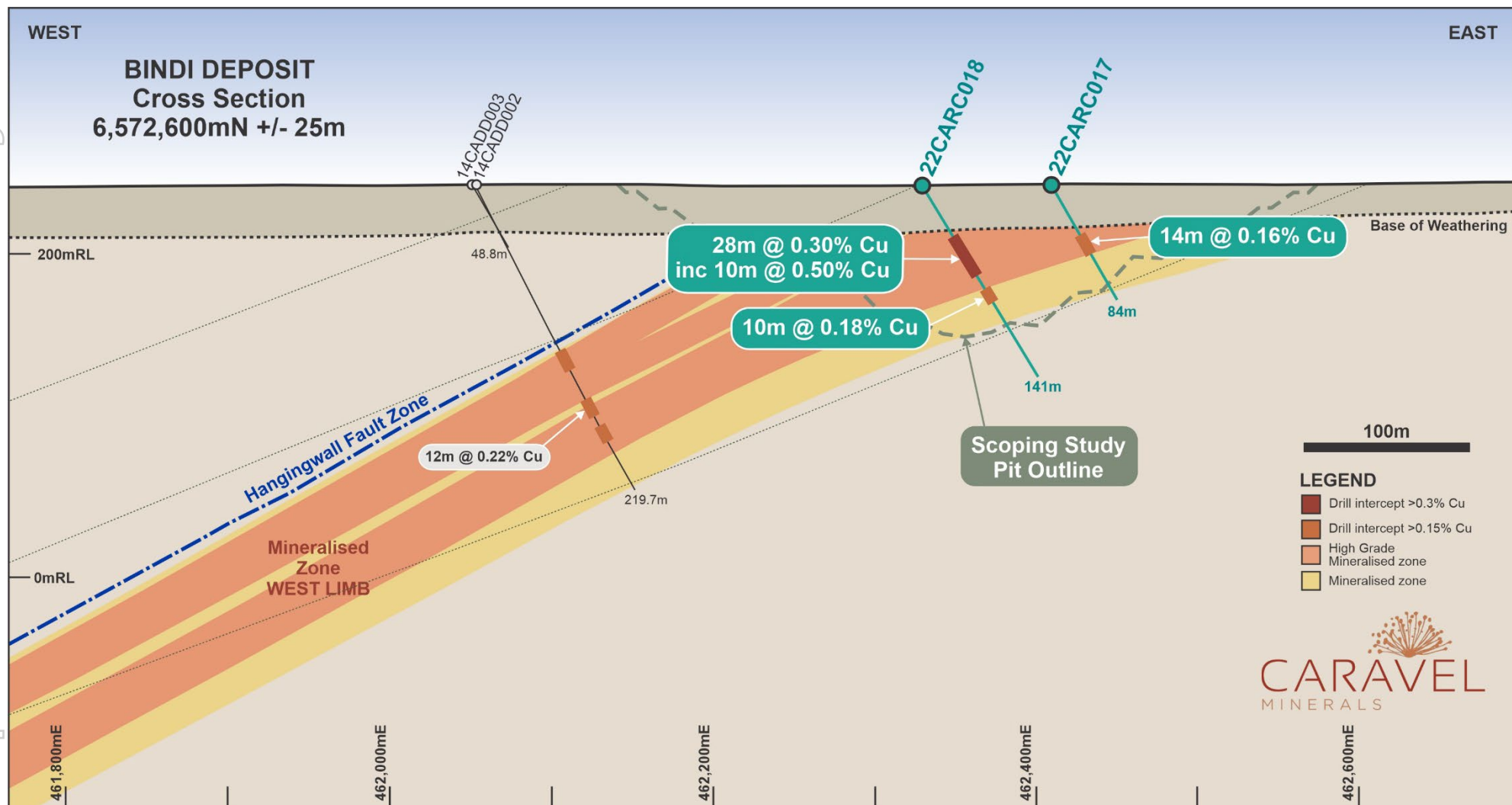
Figure 6: Schematic geological cross section of the Bindi Deposit (6,572,600mN) showing location of recent RC percussion (CARC prefix) drill holes and mineralised intersections.
