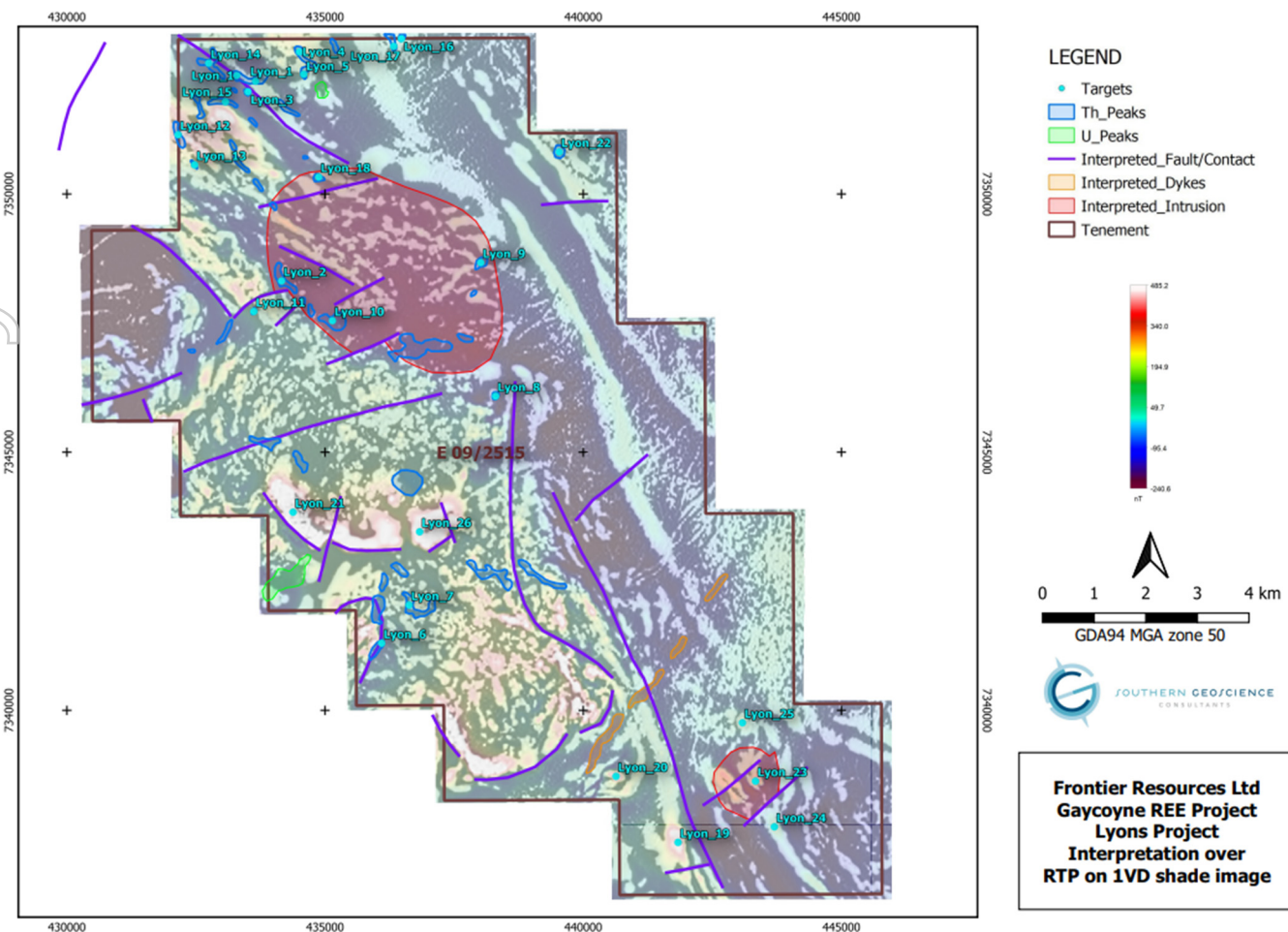
Figure 2. Frontier Resources Gascoyne REE Lyons Project Interpretation over Magnetics RTP on 1VD shade image.
