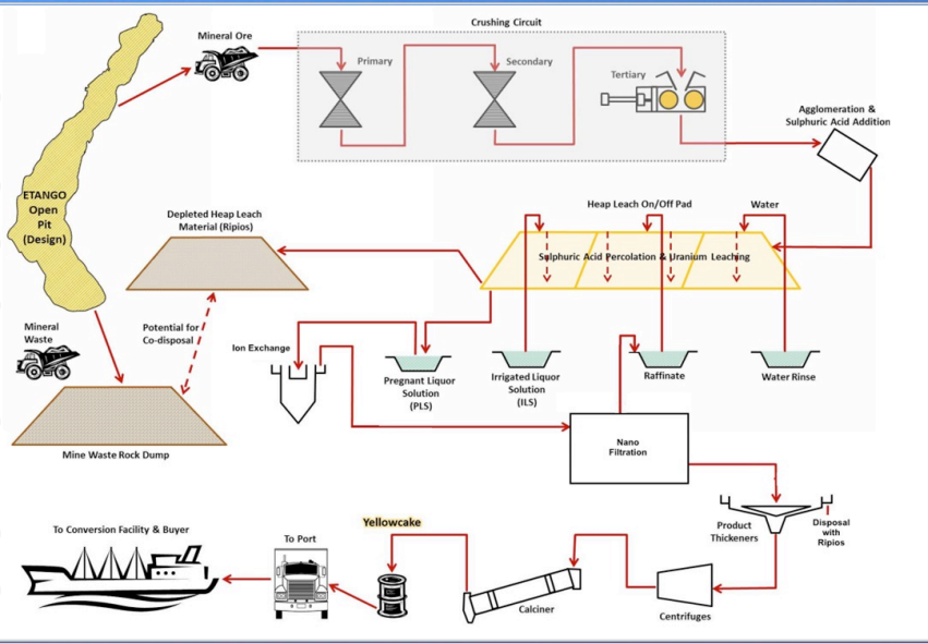
Etango-8 Flow Sheet (PFS)
