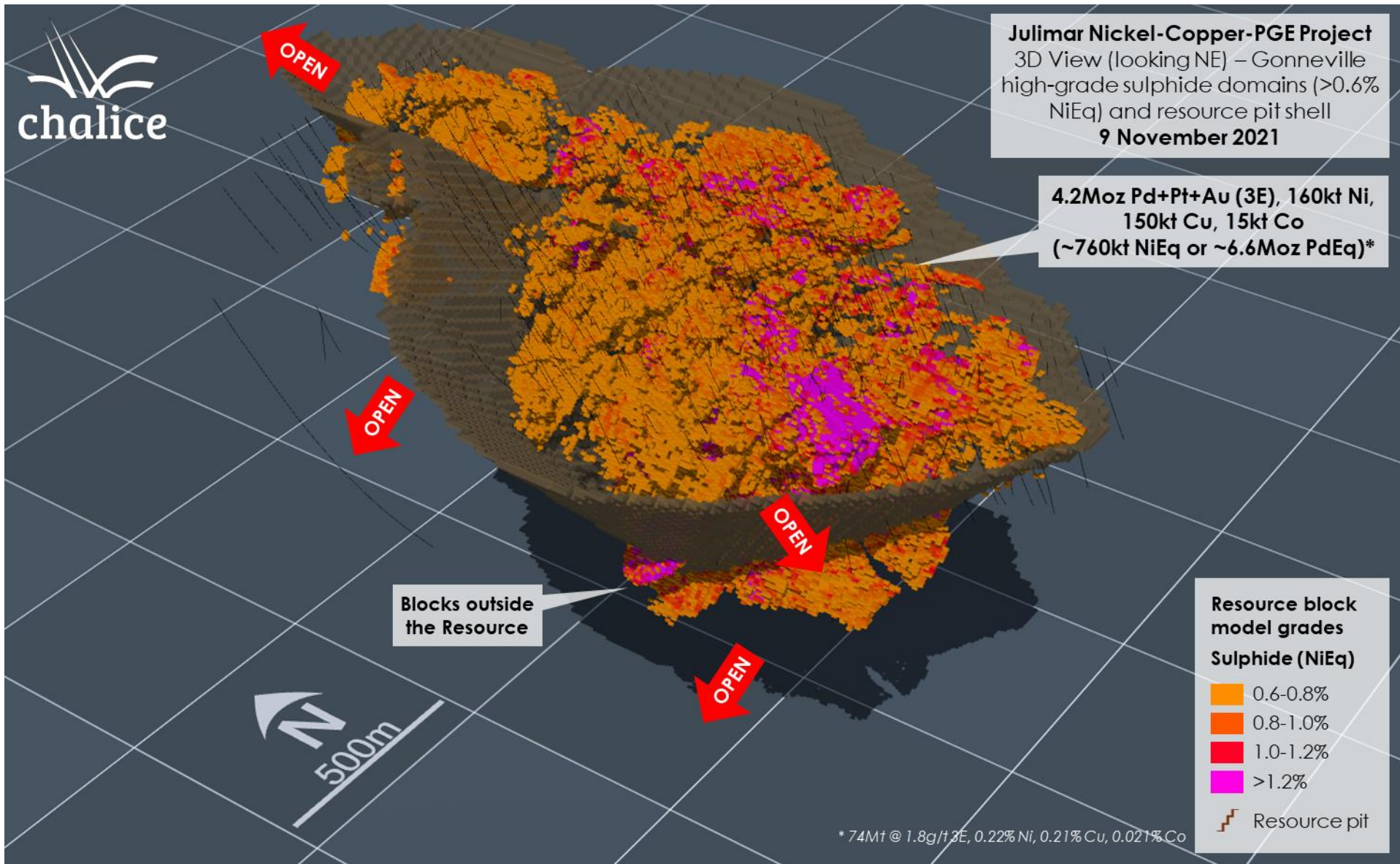
Figure 6. 3D view (looking NE) of Gonnevillie higher-grade sulphide block model (>0.6% NiEq) and Resource pit shell.
