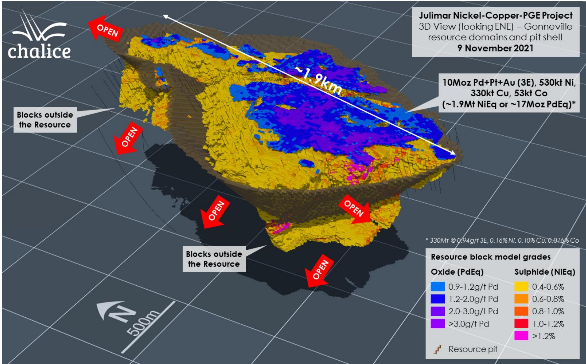
Figure 4. 3D view (looking ENE) of Gonnevillle block model (all domains) and Resource pit shell.
