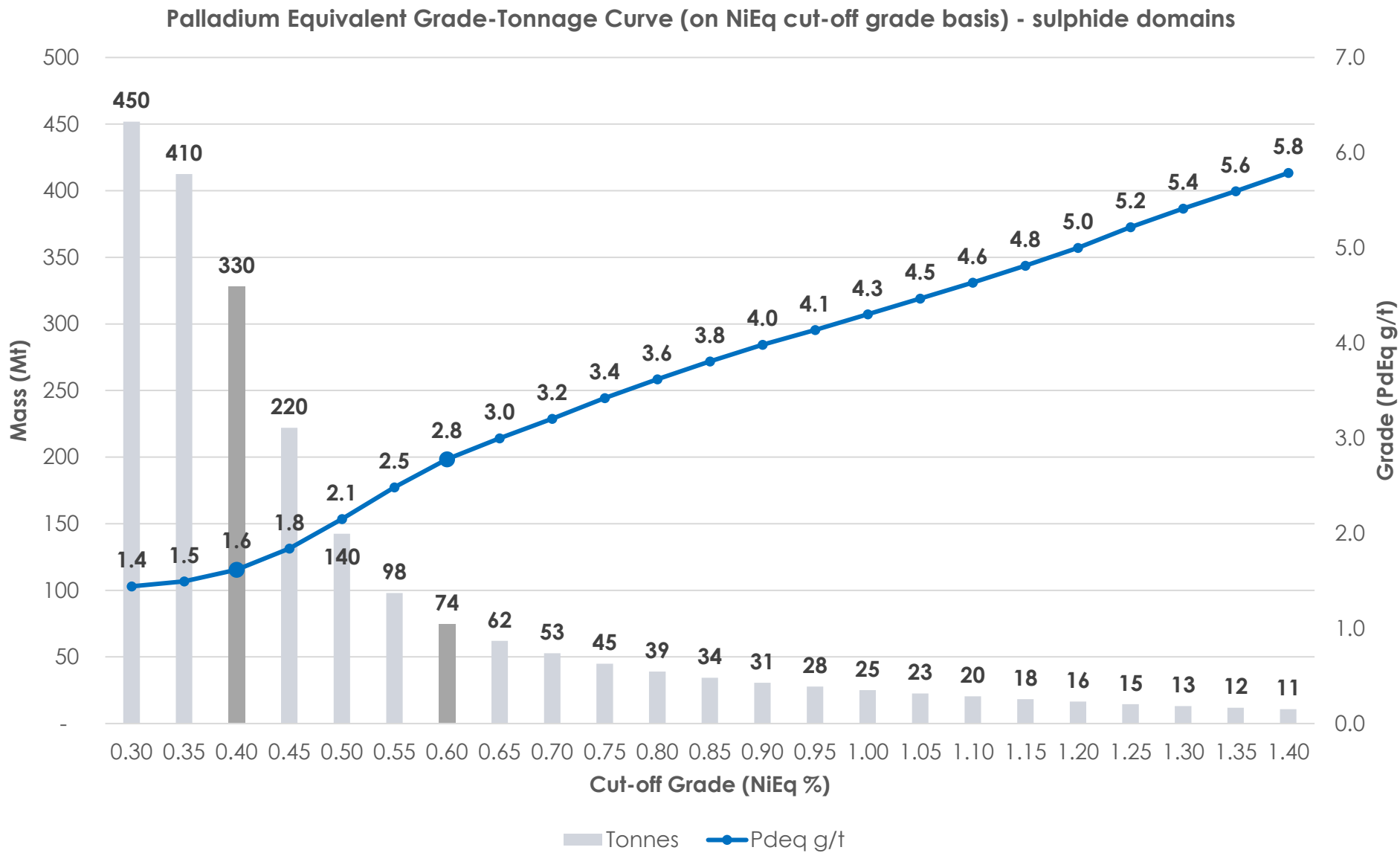
Figure 3. Gonneville PdEq grade-tonnage curve for pit-constrained sulphide mineralisation on a NiEq cut-off grade basis.
