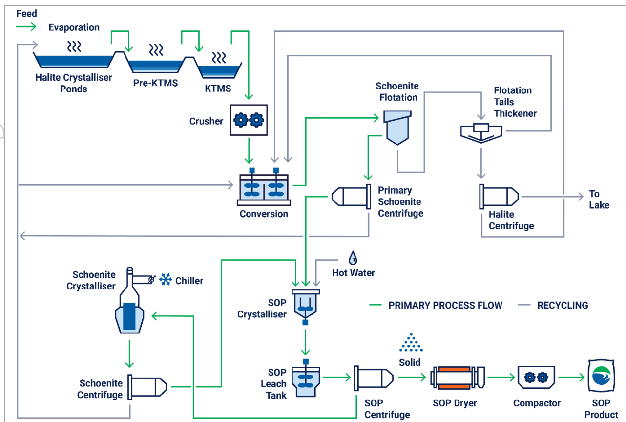
Figure 7: Flowsheet for the Lake Throssell SOP Project
