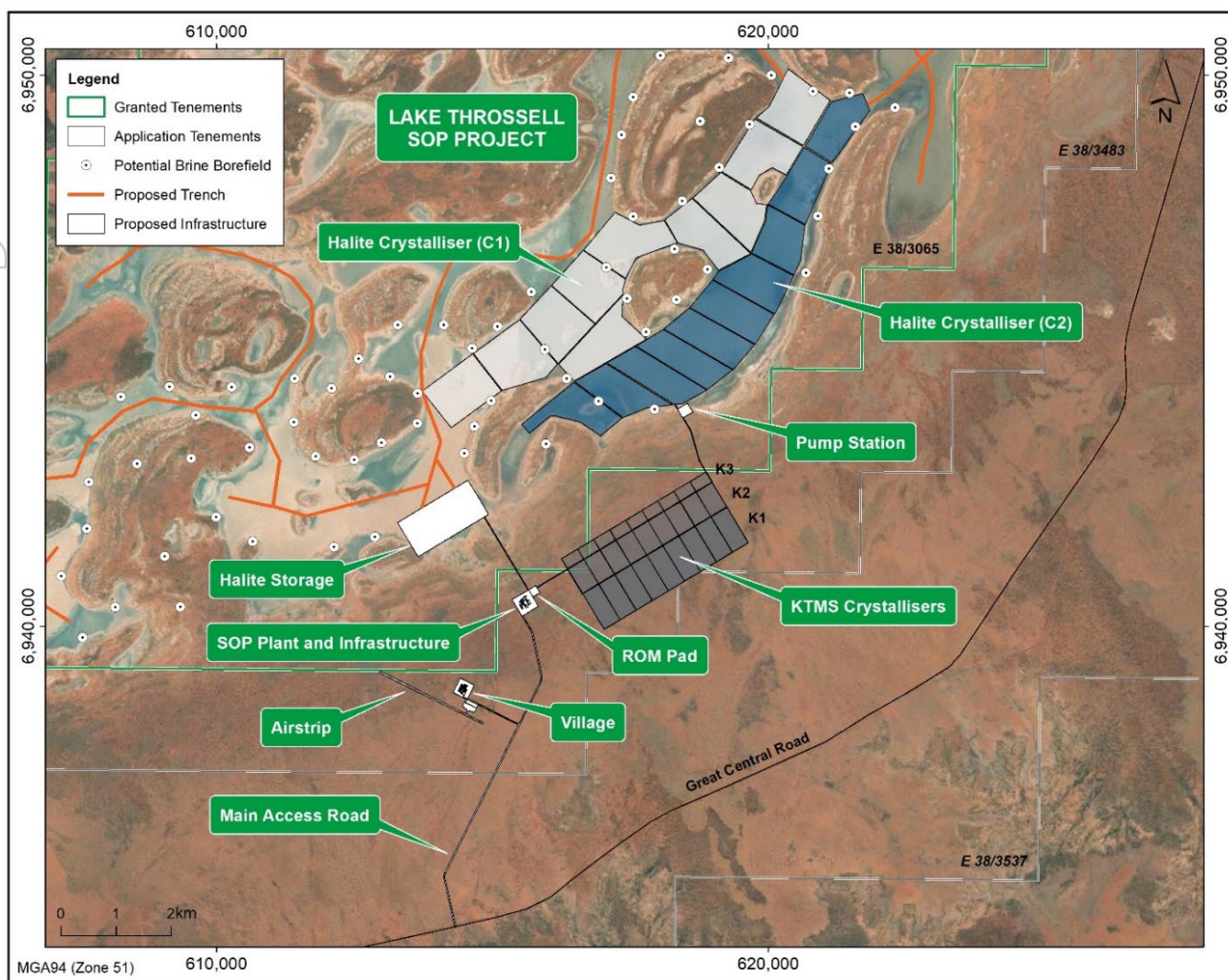
Figure 8: Indicative project layout
