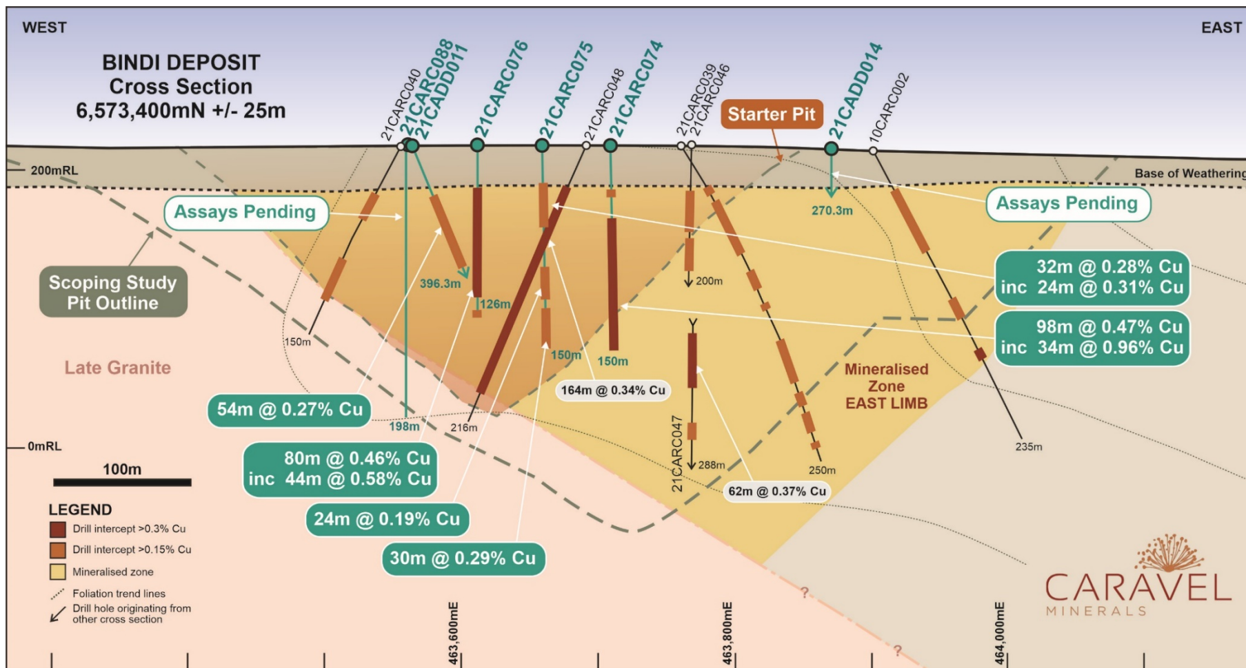
Figure 1: Schematic geological cross section of the Bindi Deposit (6,573,400mN) showing location of recent RC percussion (CARC prefix) diamond core (CADD prefix) and diamond tail (CADT prefix) drill holes and mineralised intersections.
