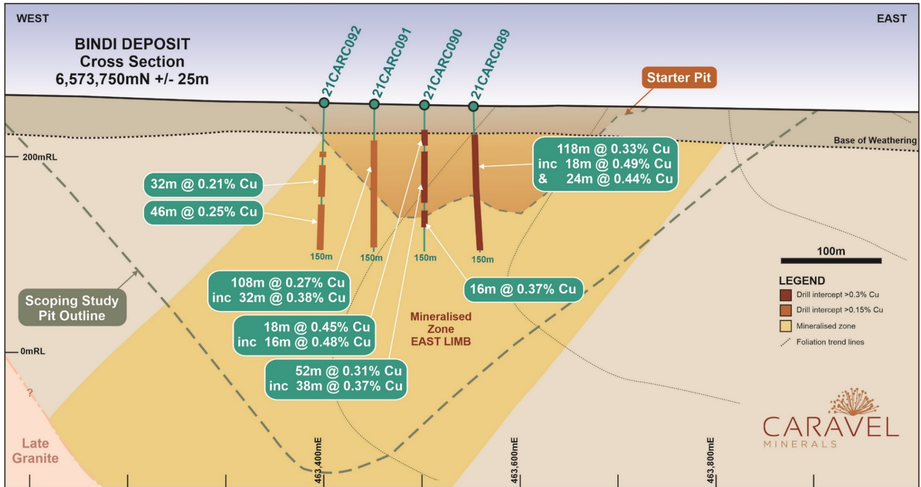
Figure 4: Schematic geological cross section of the Bindi Deposit (6,573,750mN) showing location of recent RC percussion (CARC prefix) diamond core (CADD prefix) and diamond tail (CADT prefix) drill holes and mineralised intersections.
