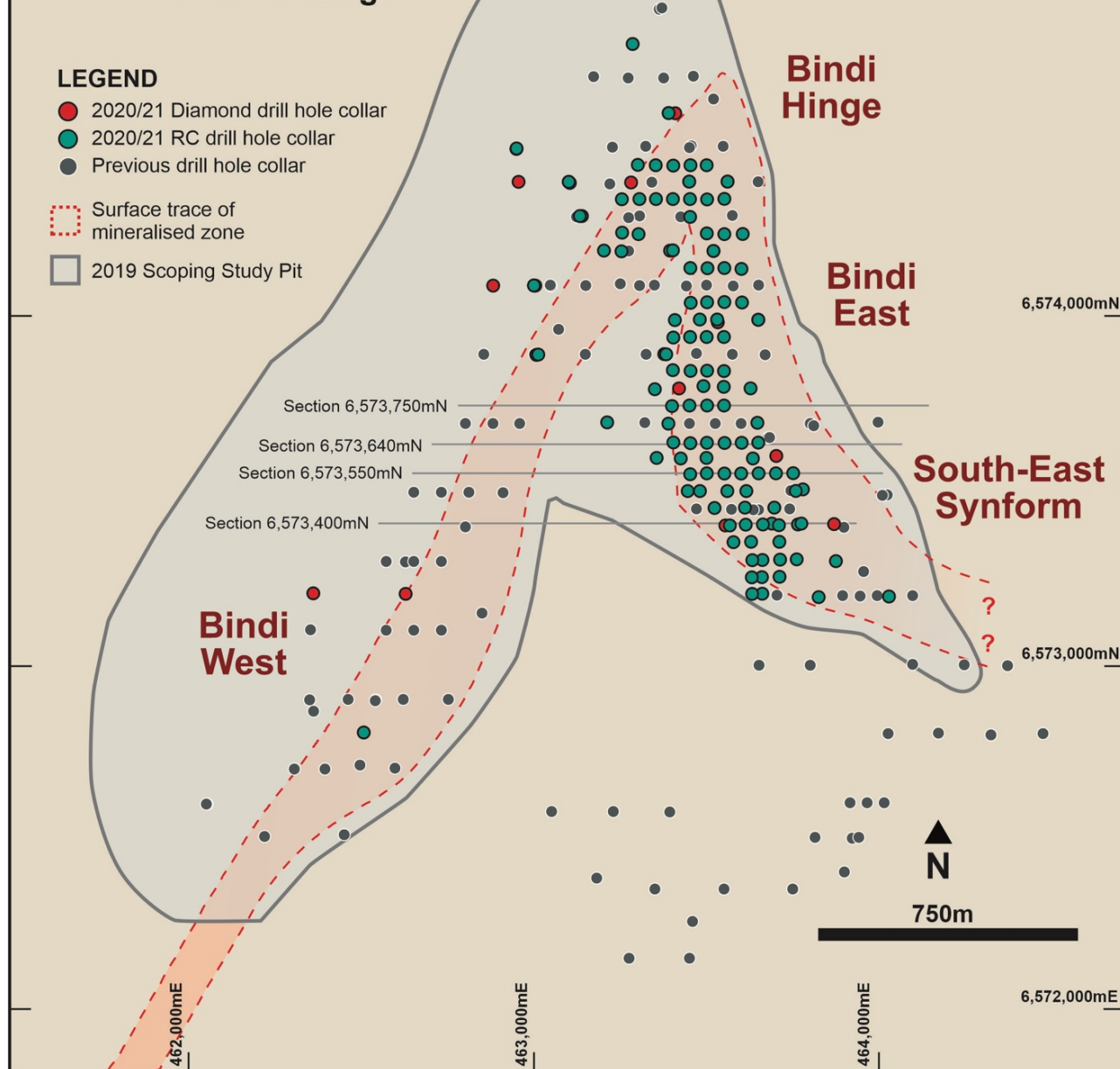
Figure 6: Drilling status plan of the Bindi copper deposit showing the locations of the reported RC percussion drill holes, drill holes from the 2020/21 program, previous drill collar locations and the 2019 scoping study pit.
