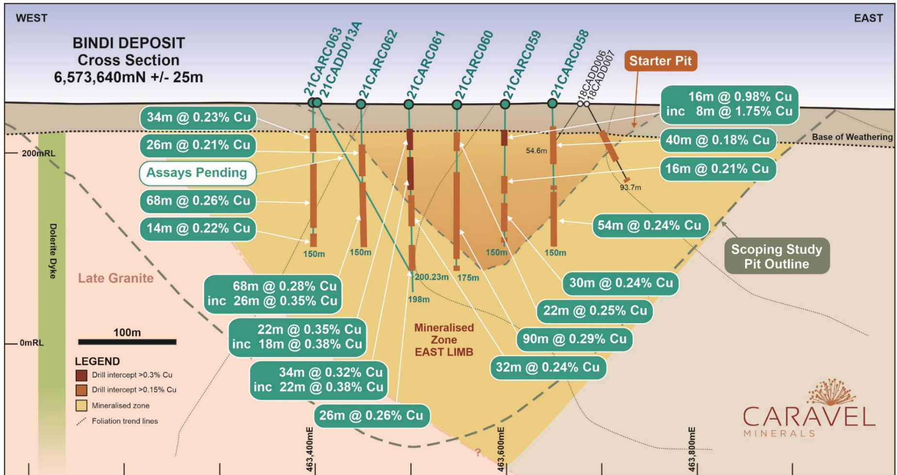
Figure 3: Schematic geological cross section of the Bindi Deposit (6,573,640mN) showing location of recent RC percussion (CARC prefix) diamond core (CADD prefix) and diamond tail (CADT prefix) drill holes and mineralised intersections.
