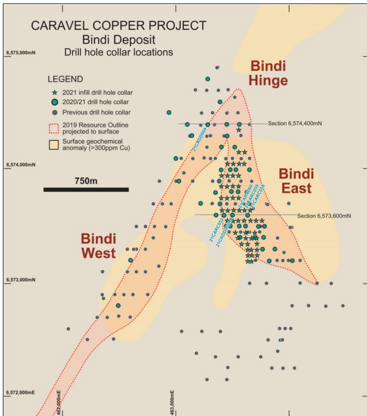
Figure 4: Drilling status plan of the Bindi copper deposit showing the locations of the reported RC percussion drill holes, previous drill collar locations and the current infill RC percussion holes.
