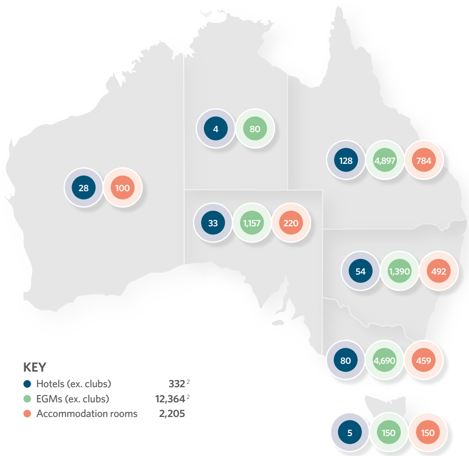
Figure 3.4.1: Hotels network 1
