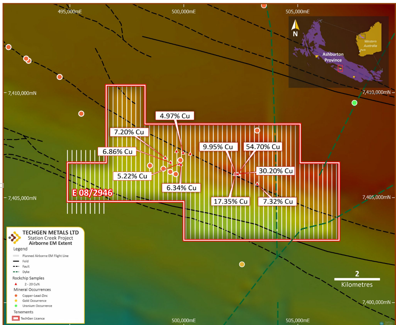
Figure 1: Station Creek Project showing planned airborne EM and peak rock chip results over airborne magnetics.
