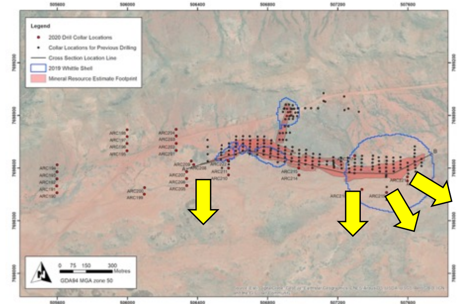
Plan View
