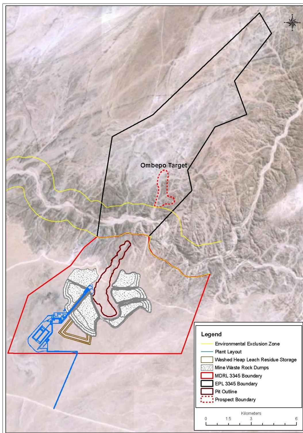
Figure 1: The Etango uranium project, showing licence boundaries of EPL 3345 and MDRL 3345
