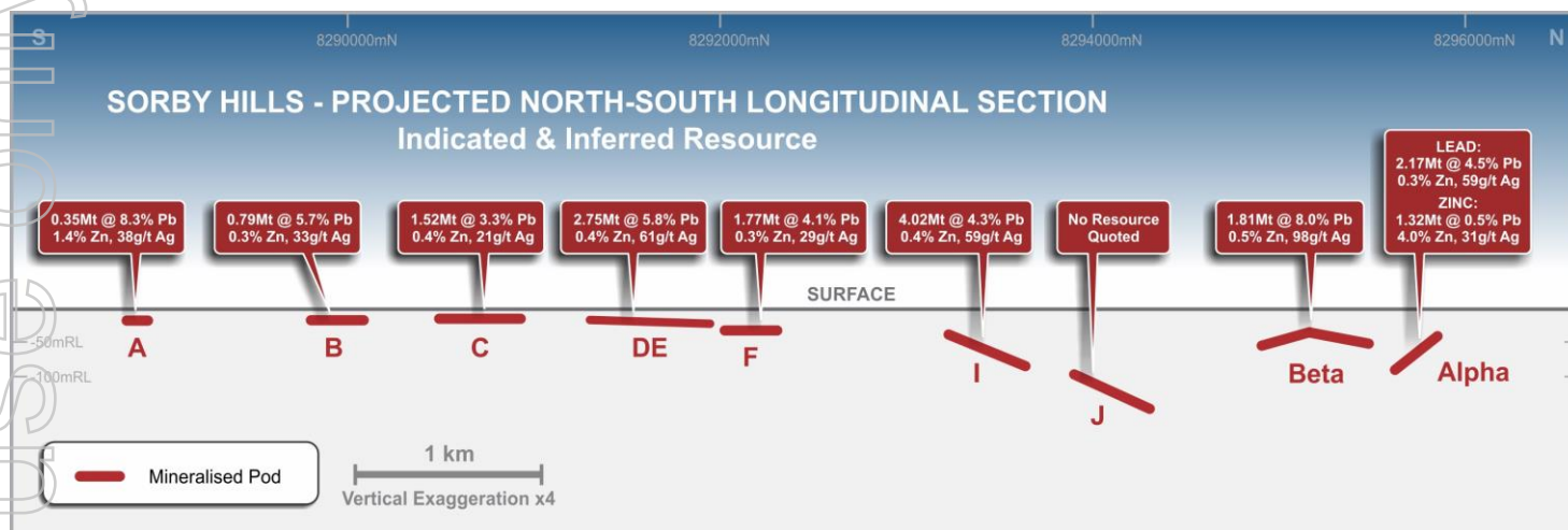
Figure 2. Sorby Hills Long Section (Looking West) Showing a Schematic of the Deposits.
