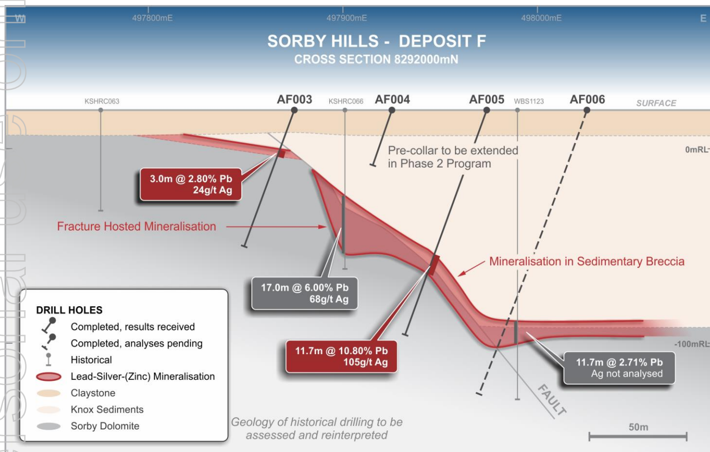
Figure 5. F Deposit: A Fault Defines the Contact of Knox Sediment and Sorby Dolomite. Pacifico Down Hole Intersections Shown in Red.
