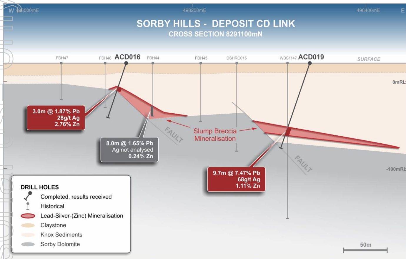
Figure 6. CD Link: Pacifico Down Hole Intersections Shown in Red.
