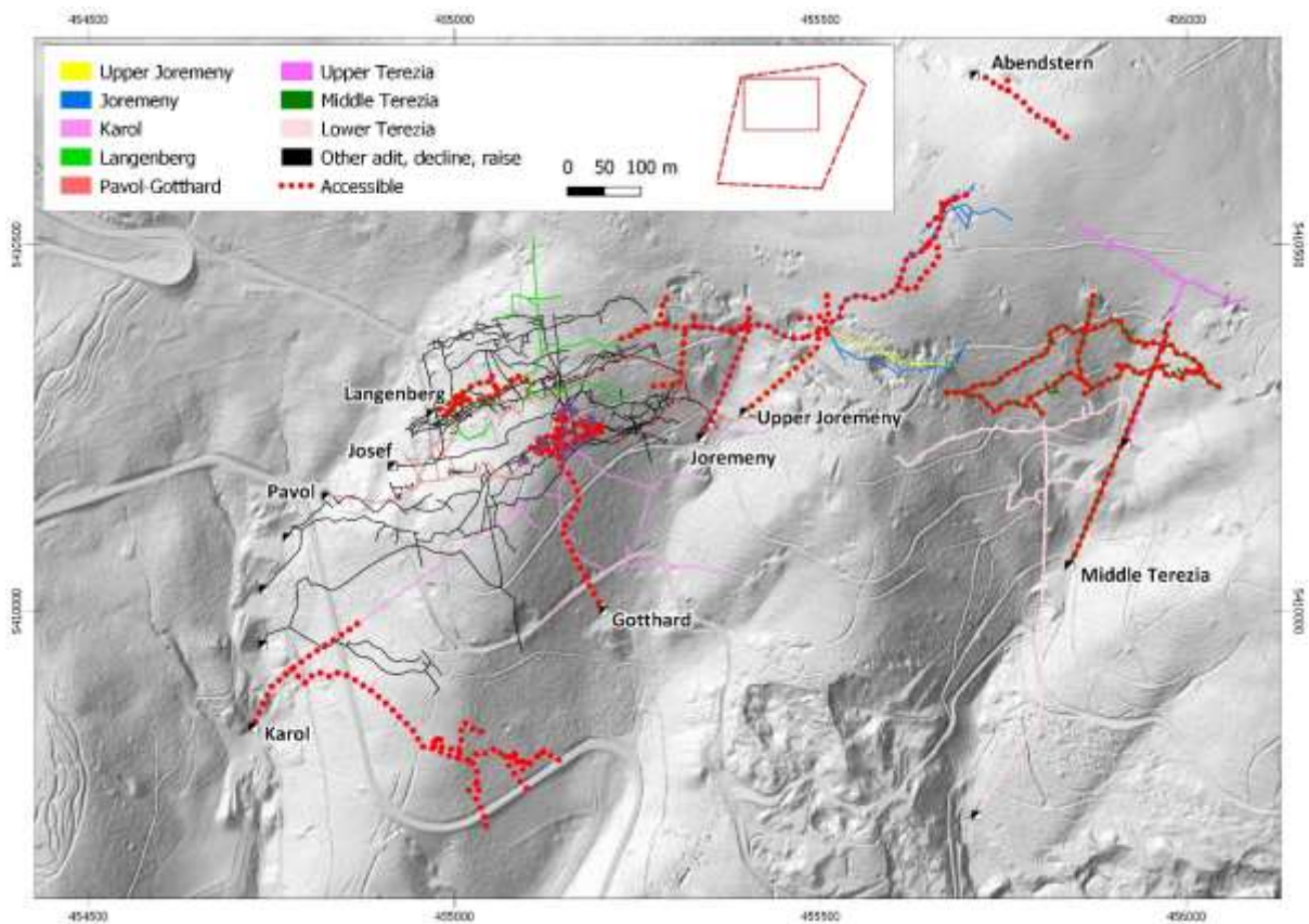
Figure 3: Plan View of Zemberg-Terezia Adits and Areas Accessible
