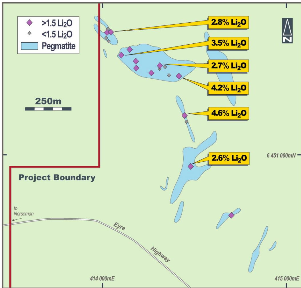
Figure 1: Buldania Project – Plan showing approximate pegmatite locations and Liontown rock chip samples
