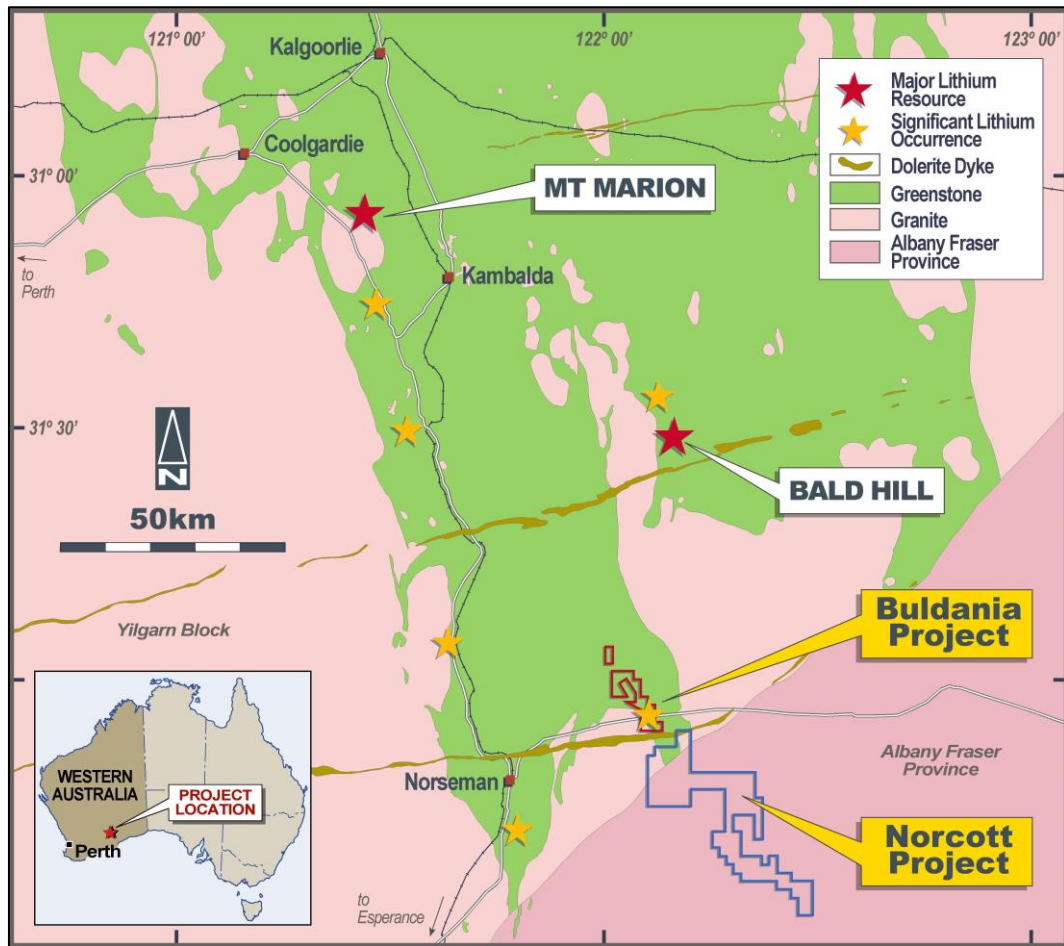
Figure 3: Plan showing regional geology, lithium occurrences and Liantown Projects
