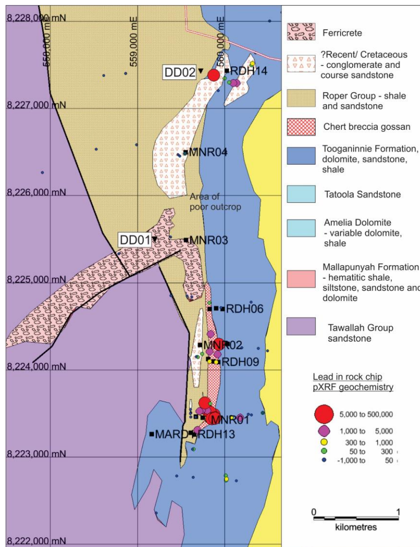
Mariner –geology, previous percussion drilling, Pacifco 2016 RC collars, and planned 2017 diamond drill sites (DD01 and DD02)
