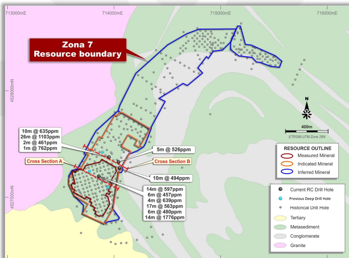
Figure 1: Drilling Plan
