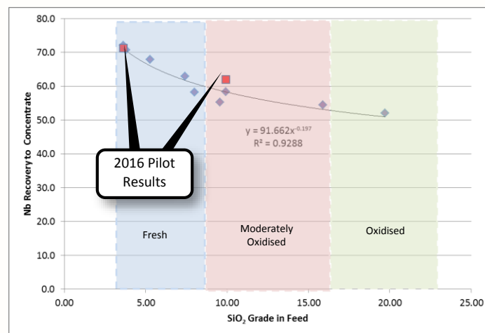
Niobium Recovery Trend by Geological Zone (SiO 2 Grade in Feed)
