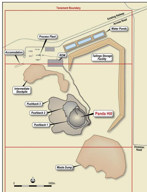
Figure 8 – Site layout
