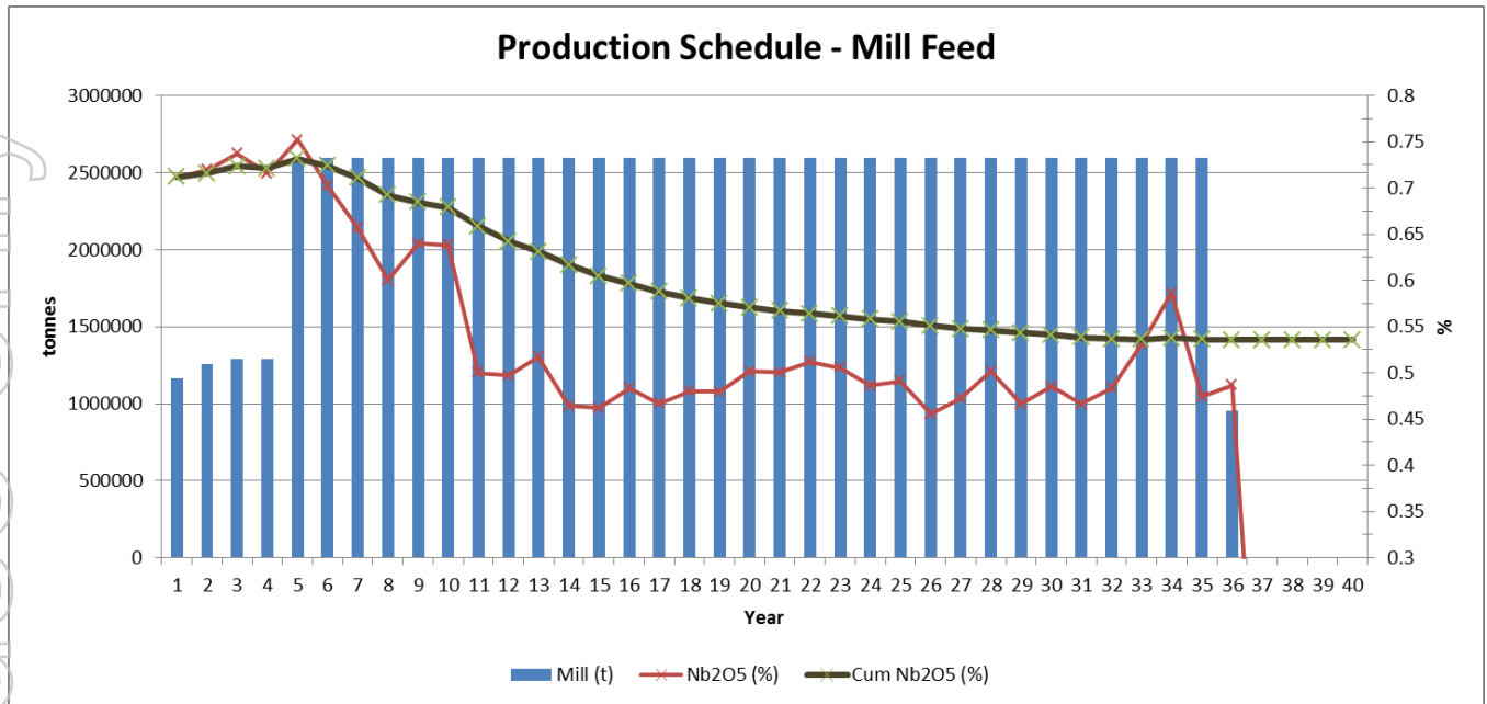
Figure 4 – Panda Hill Production Schedule
