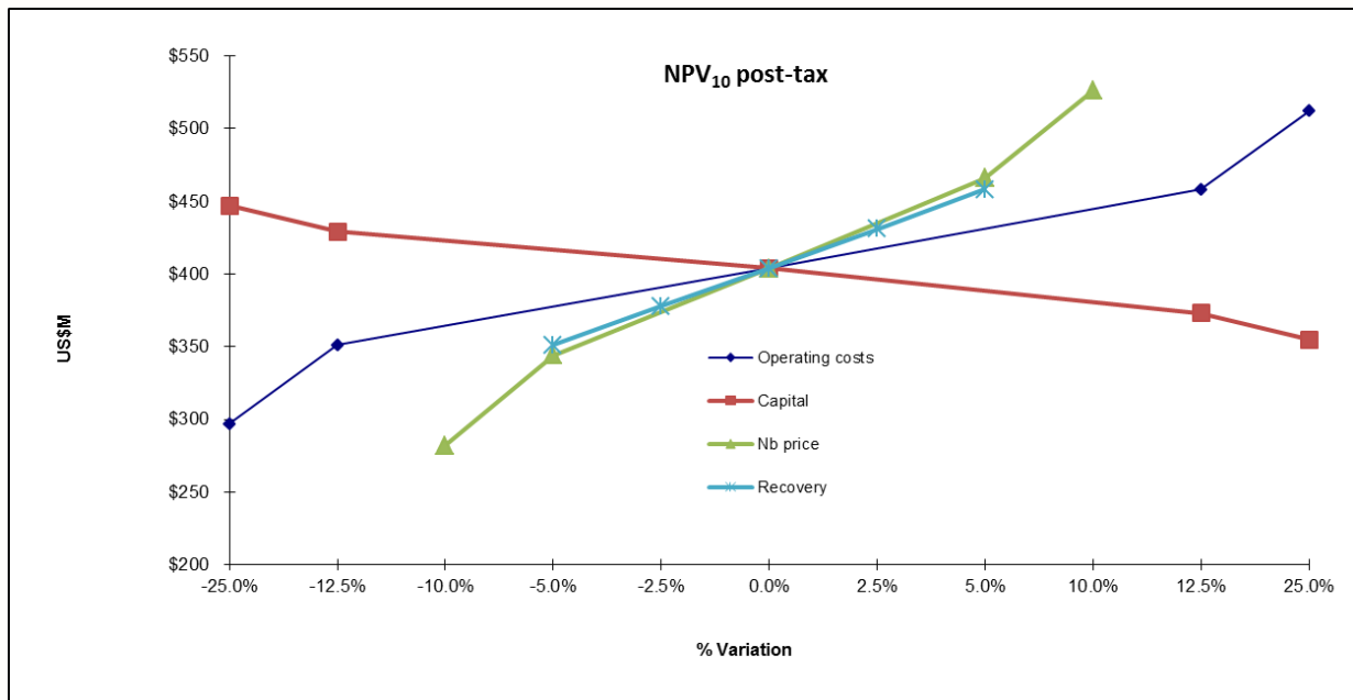
Figure 19 – Sensitivity analysis of key economic drivers
