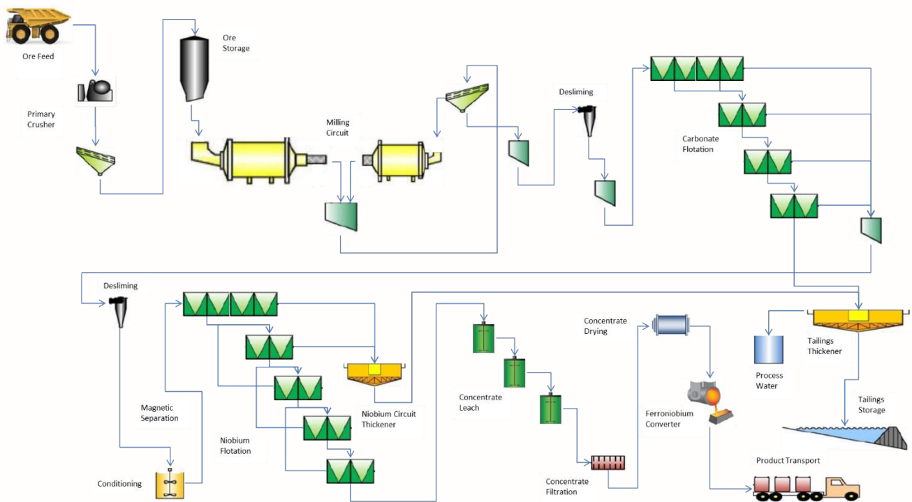
Figure 6 – Schematic of proposed flowsheet
