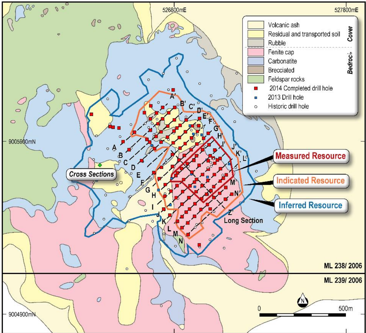
Figure 3 – Geology plan showing the 2015 Mineral Resource regions and drilled section lines. The regions in blue (carbonatite) and pink (Fenite Cap) are both highly prospective with field mapping showing carbonatite and magnetite-carbonatite outcrop contained within many of these areas. Cradle has only drill tested approximately 40% of the area of the carbonatite, with the remaining areas having mineralisation indicated by historical drilling.
