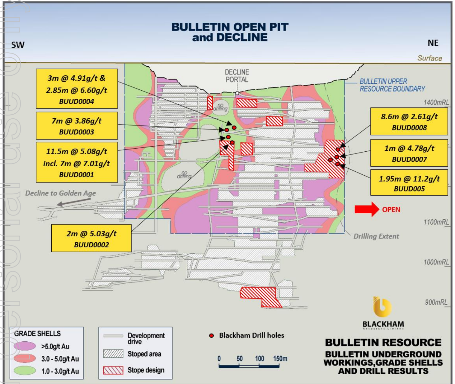
Fig 1. Long-section looking North West of Bulletin underground workings, grade shells and current resource outline.
