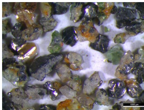
Figure 2b sample from Namangale 1 showing mostly liberated graphite flakes up to 1000 microns in size
