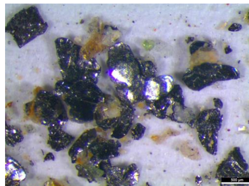
Figure 2c sample from Namangale 1 showing well liberated graphite flakes
