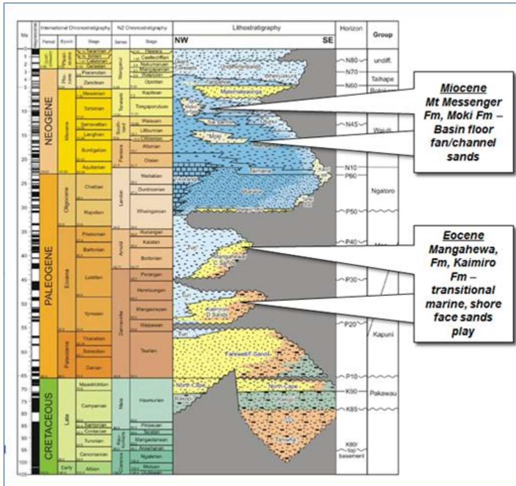
Figure 5-1 Taranaki Basin stratigraphic column
