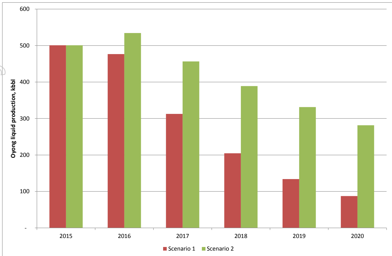
Figure 6-8: Oyong valuation case oil forecasts (untruncated)
