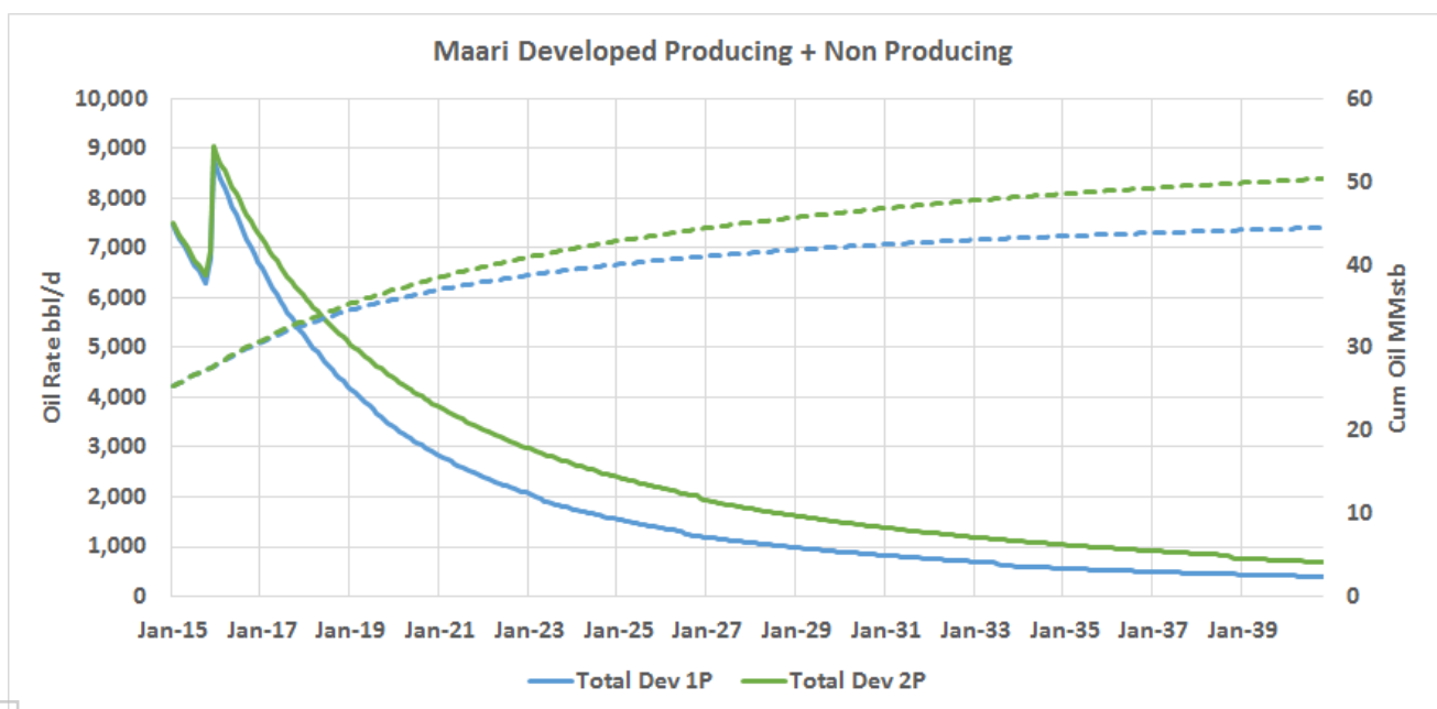
Figure 5-5 Maari Developed Production Forecast
