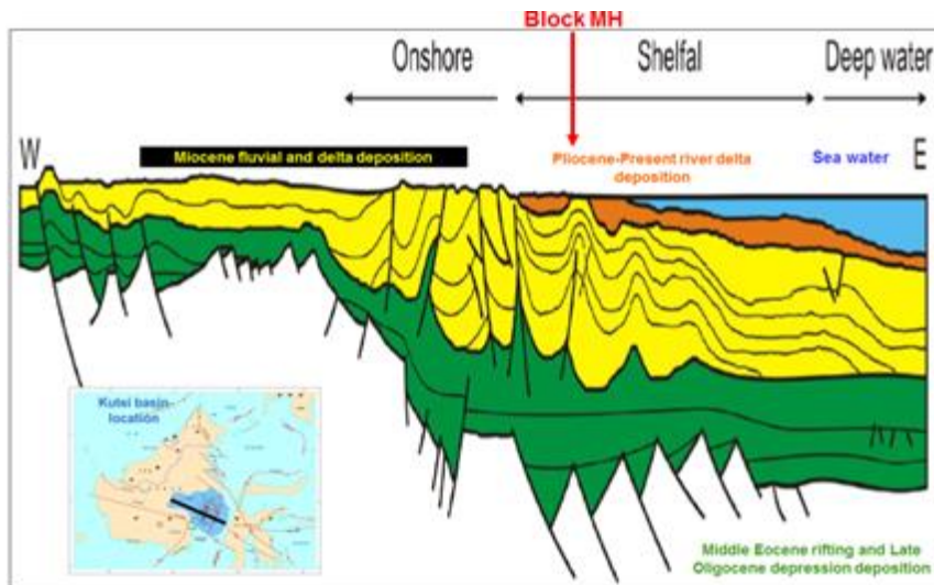
Figure 6-14: Kutei Basin cross section
