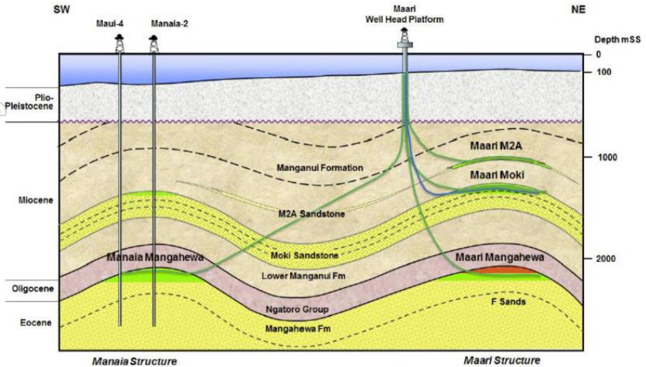
Figure 5-3: Maari Manaia Structural Section
