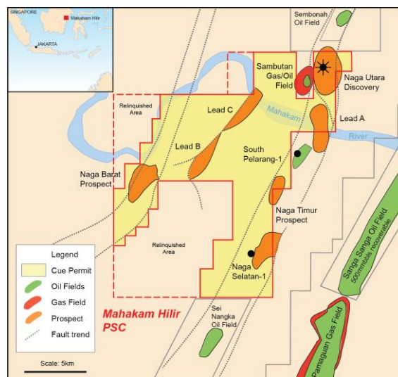
Figure 6-15 Mahakam Hilir PSC prospects, leads and adjacent fields.
