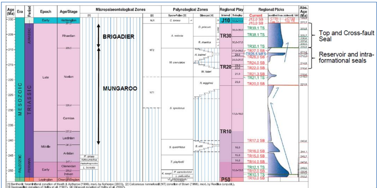
Figure 7-4: Northern Carnarvon secondary petroleum system
