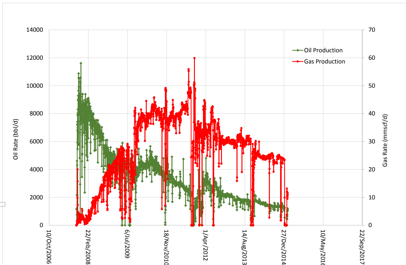
Figure 6-7: Oyong Historical Production Performance
