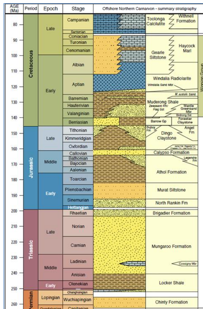
Figure 7-2: Northern Carnarvon Basin stratigraphic column
