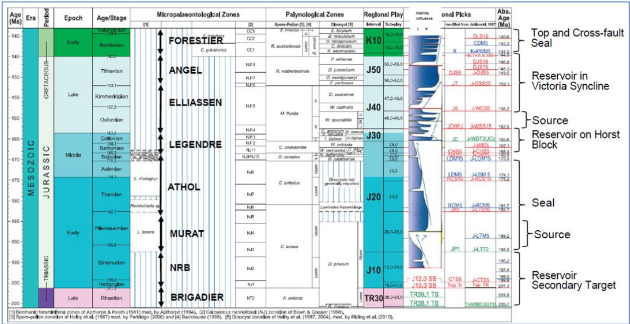
Figure 7-3: Northern Carnarvon primary petroleum system
