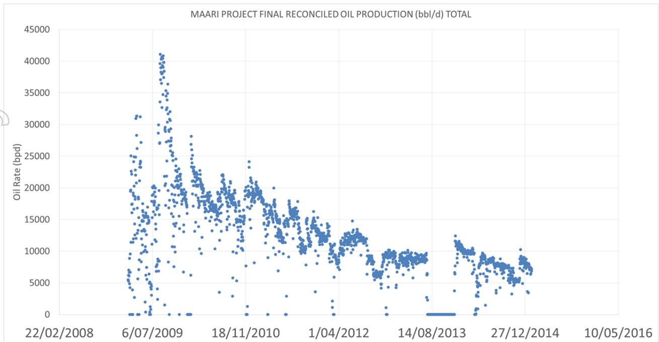
Figure 5-4 Maari Production History
