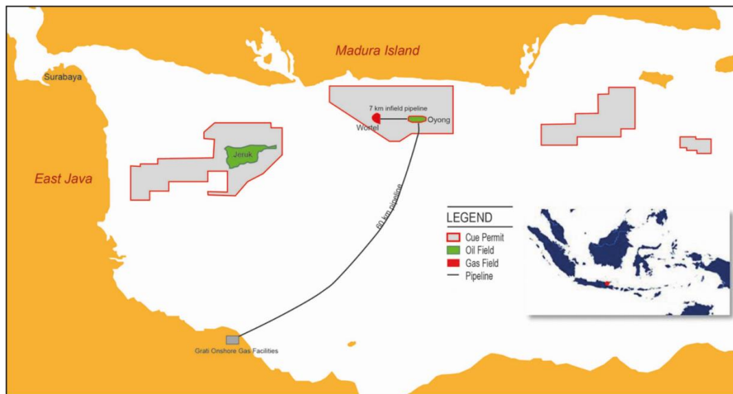
Figure 6-1: Wortel and Oyong location and gas flowlines
