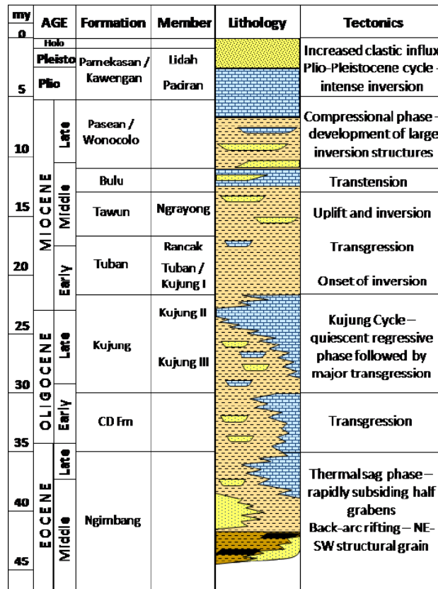
Figure 6-2: General stratigraphic column for the East Java Basin
