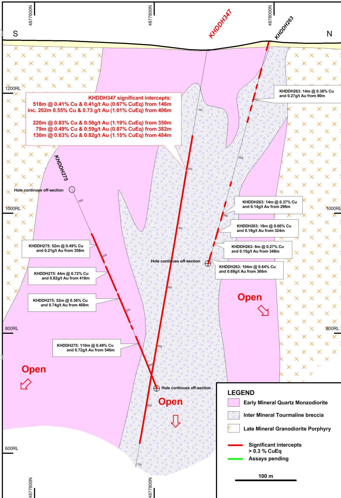
FIGURE 2: KHDDH347 CROSS SECTION
