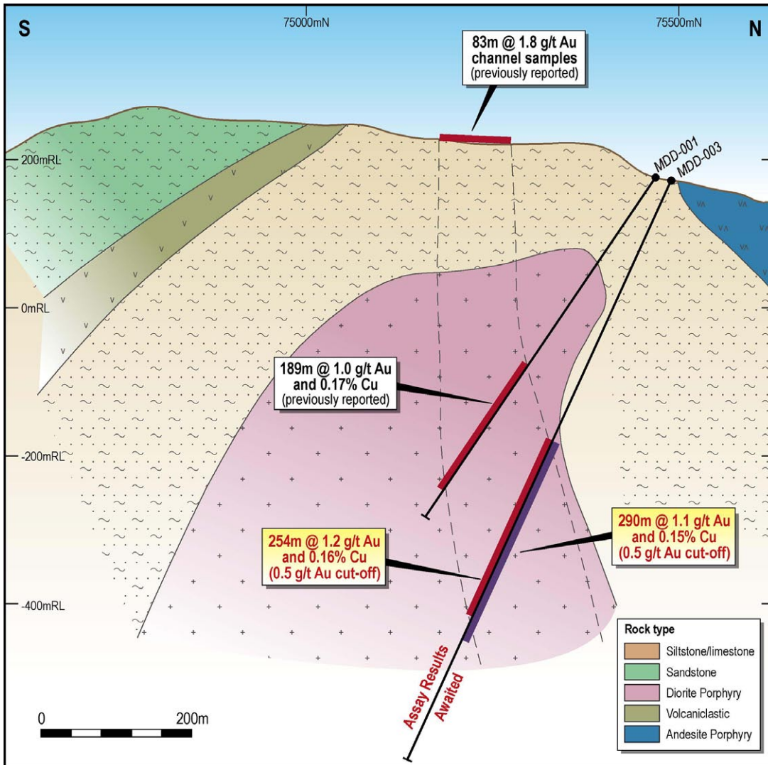
Section 77850mE showing MDD003 drilling result and interpreted geology.
